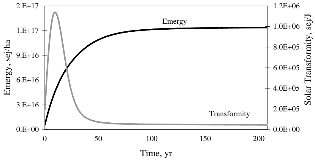
Figure 22. Emergy and transformity of forest biomass storage in forested wetland model.
