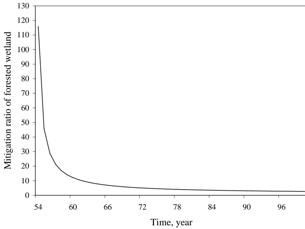
Figure 29. Simulated mitigation ratios for forested wetlands from 54 to 100 years after construction showing decrease in mitigation ratios as the time frame allowed to offset losses increases.
