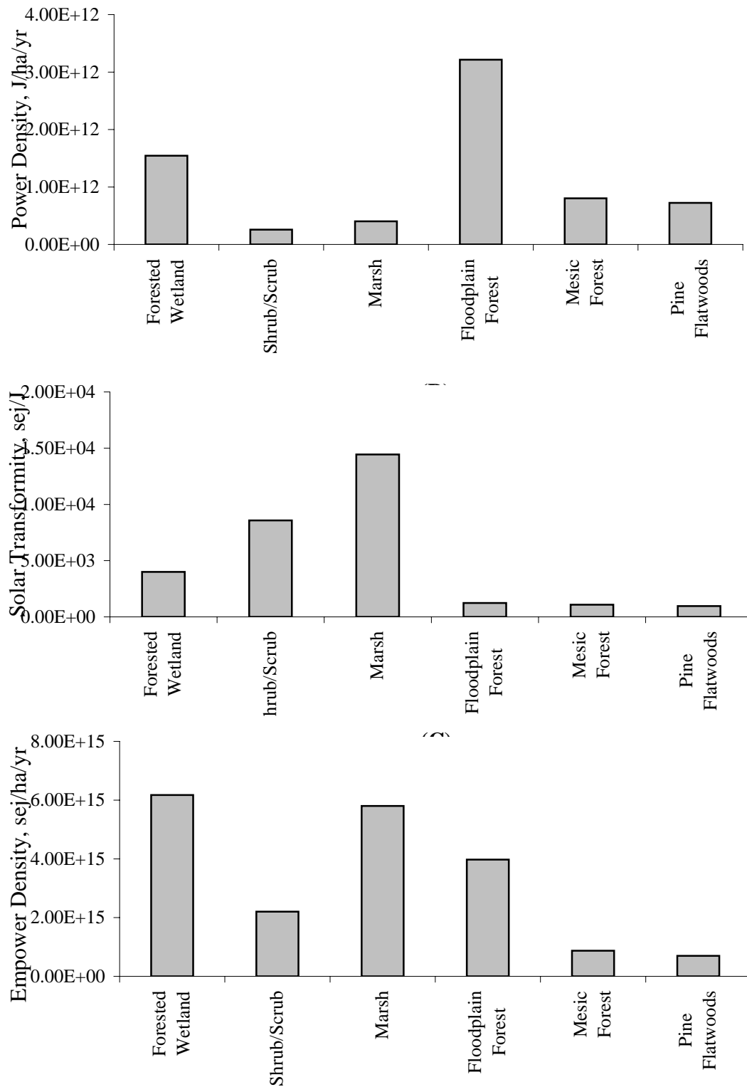
Figure 13. GPP values of six Florida ecosystems. (A) Power Density; (B) Solar Transformity; (C) Empower Density. See Appendix B, Tables 10-21.
