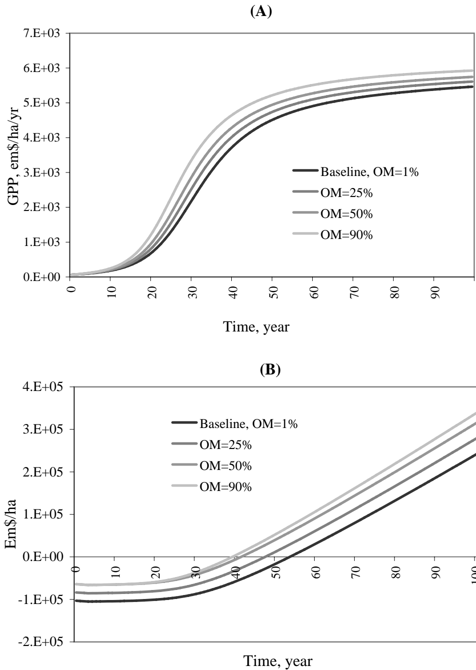
Figure 27. Simulation results of GPP and recovery time under different initial organic matter storage values, showing an increase in GPP (A) and a decrease in recovery time (B) as the initial organic matter storage is increased by 25%, 50% and 90% of its steady state value.
