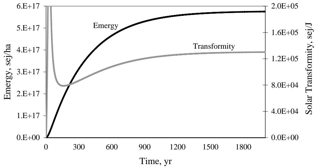
Figure 23. Emergy and transformity of organic matter storage in forested wetland model.
