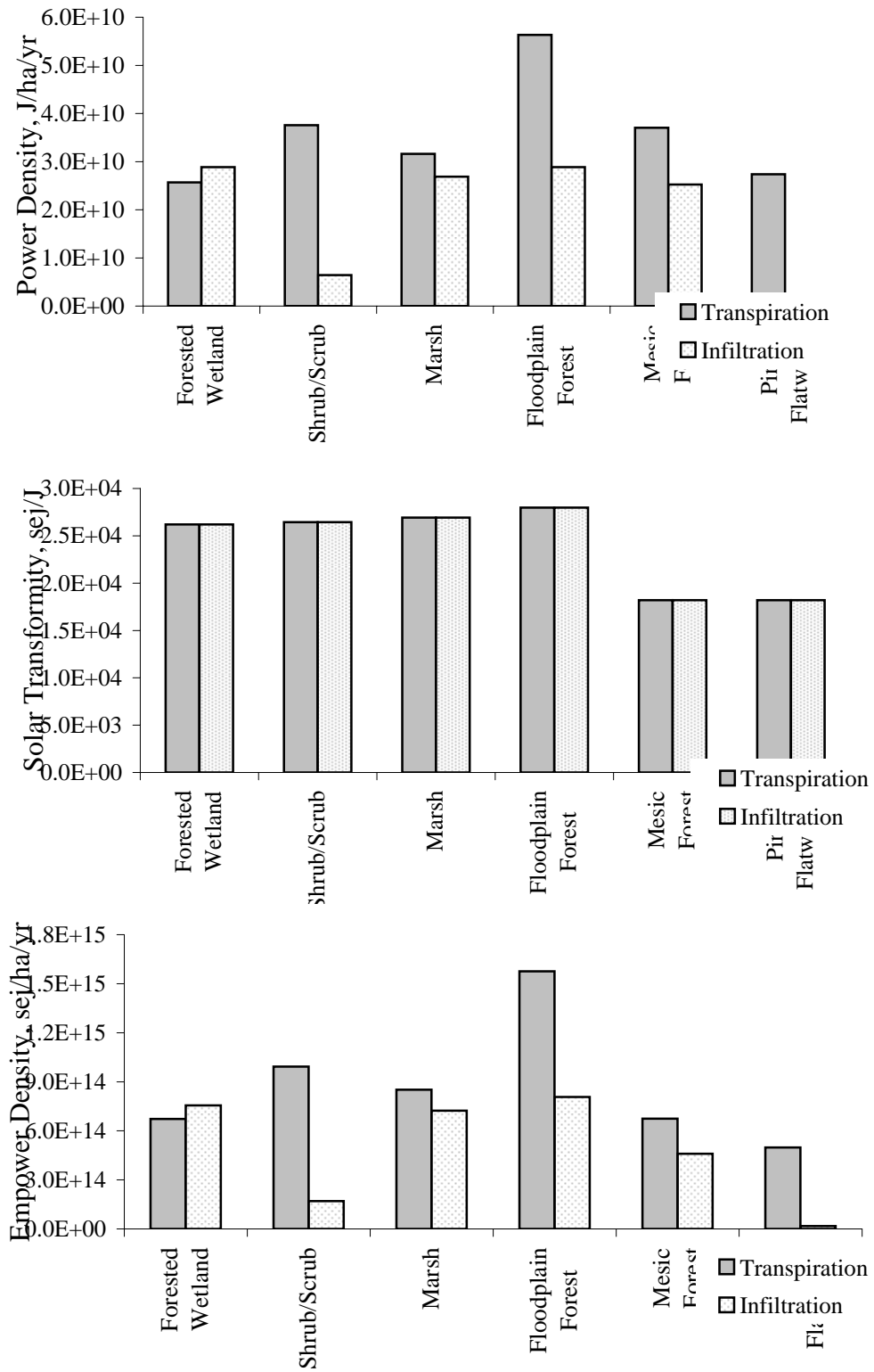
Figure 12. Transpiration and infiltration values of six Florida ecosystems. (A) Power Density; (B) Solar Transformity; (C) Empower Density. See Appendix B, Tables 10-21.
