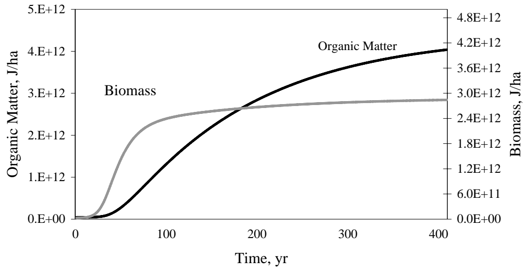
Figure 21. Simulation results of the forested wetland model showing time series of forest biomass and organic matter storages.
