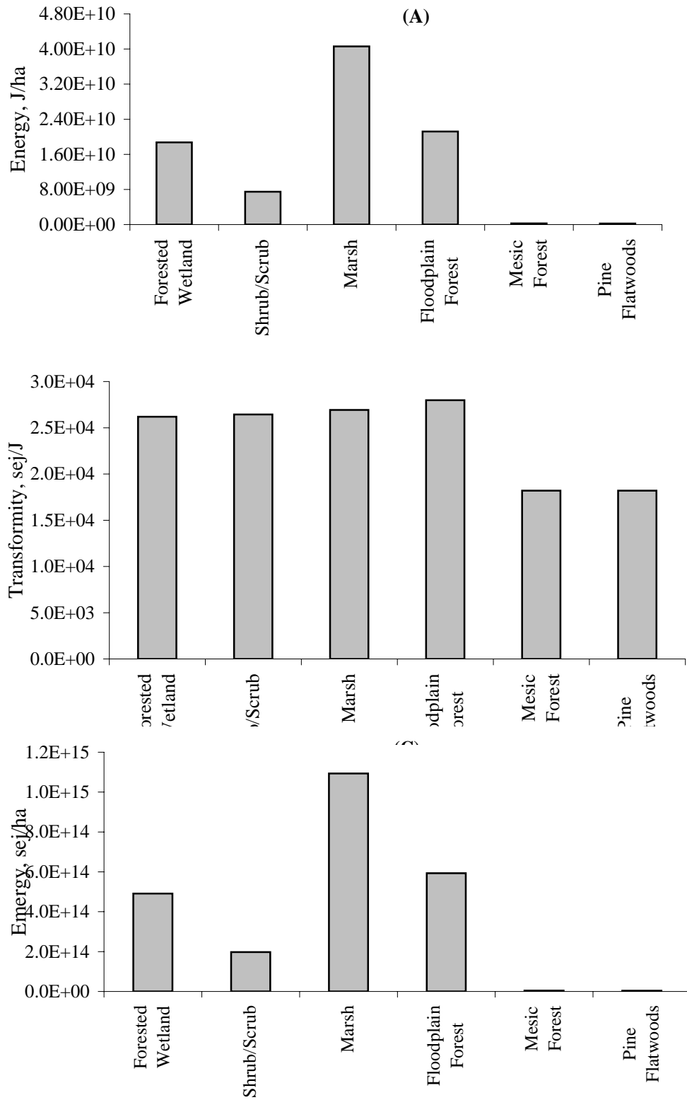
Figure 16. Soil water values of six Florida ecosystems. (A) Energy; (B) Transformity; (C) Energy. See Appendix B, Tables 10-21.
