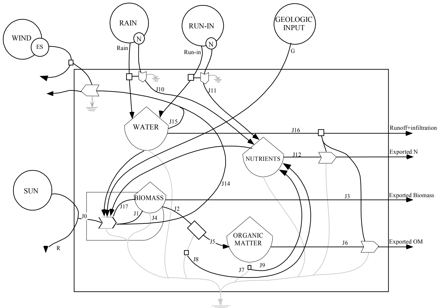
Figure 18. Systems diagram of the forested wetland simulation model showing energy flows and storages evaluated.
