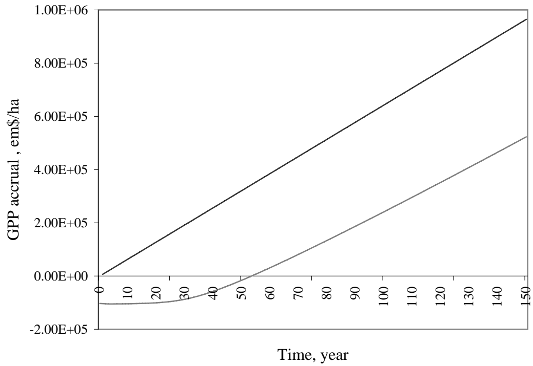
Figure 28. Graph of GPP accrual in mature forested wetland and constructed ecosystem. The ratio of these two lines at any point in time constitutes the mitigation ratio necessary to recover losses due to construction within that time frame.
