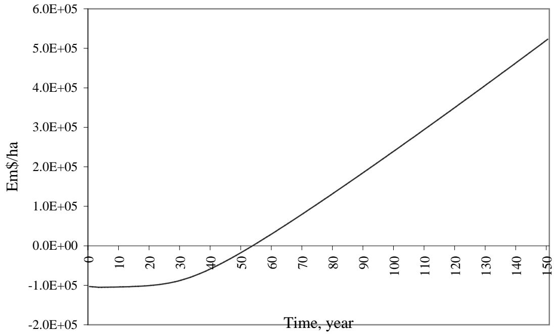
Figure 26. Simulation of (A) GPP emdollar value and (B) recovery time needed to payback construction costs (calculated by adding yearly GPP to initial debt).
