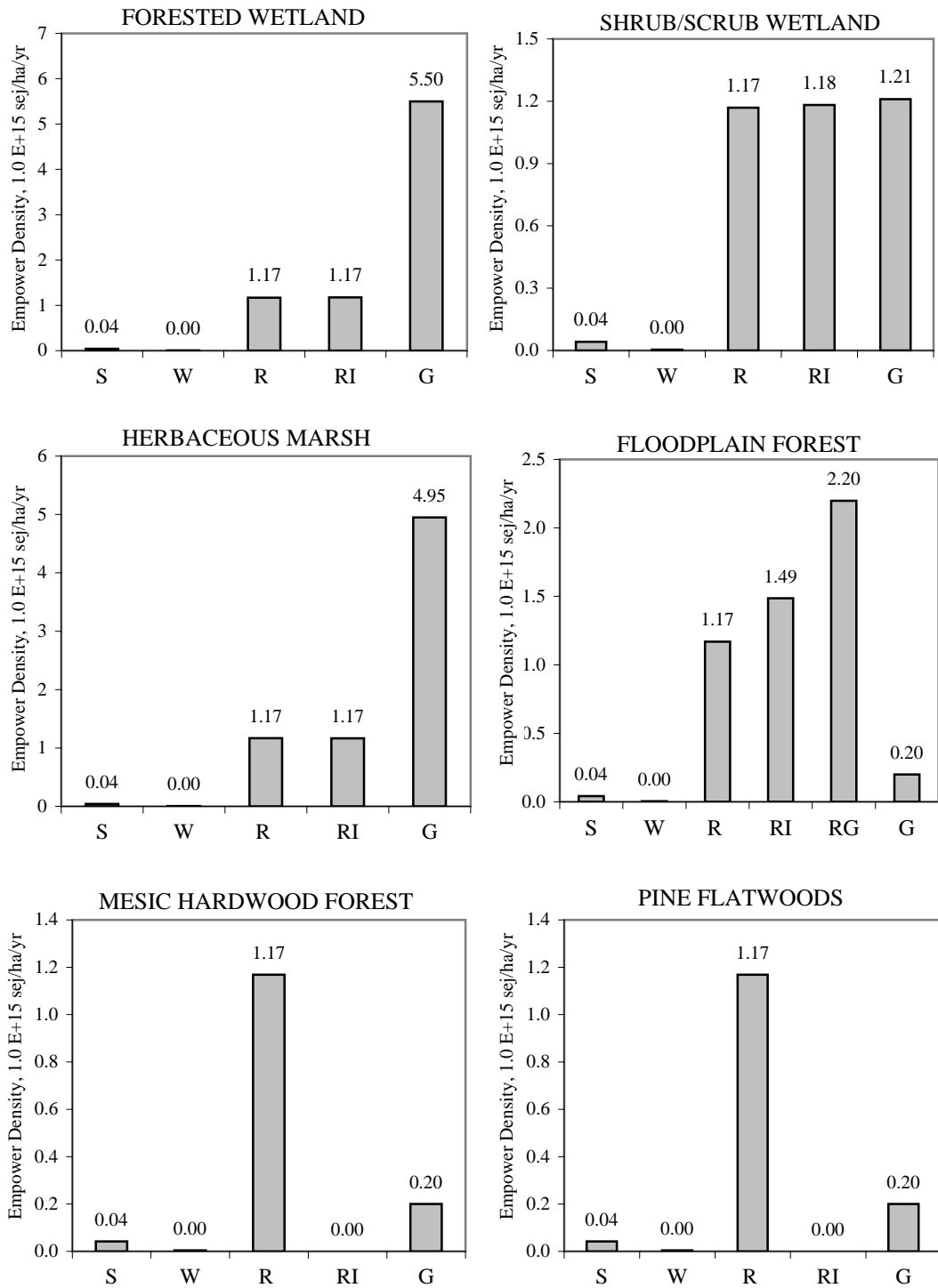
Figure 10. Emergy signature of six Florida ecosystems showing the environmental inputs to the system. S = sun; W = wind; R = rain; RI = run-in; G = geologic input; RG = river geopotential. Note the different scale on each graph. Calculated from data in Appendix B, Tables 10-21.
