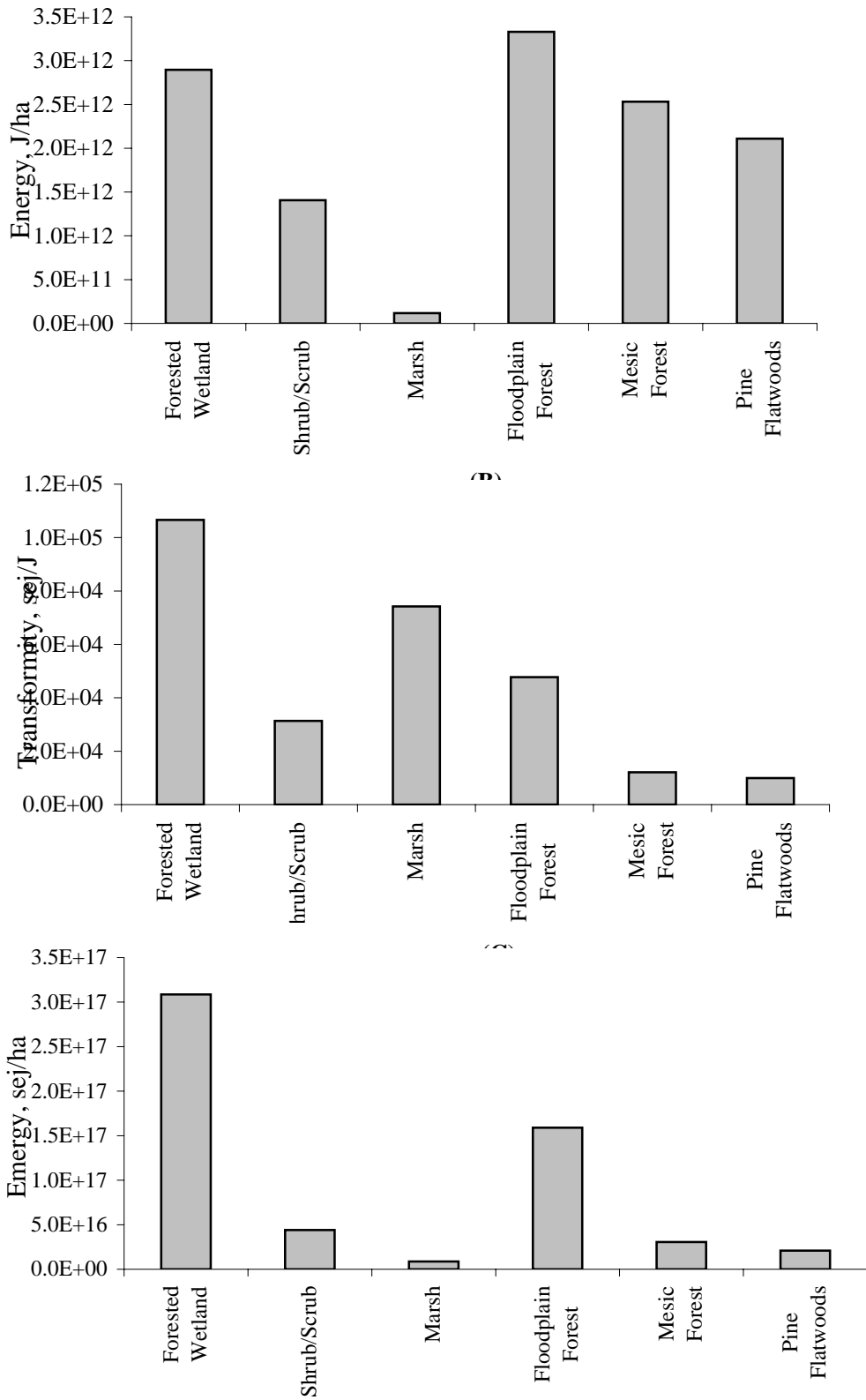
Figure 14. Biomass values of six Florida ecosystems. (A) Energy; (B) Transformity; (C) Energy. See Appendix B, Tables 10-21.
