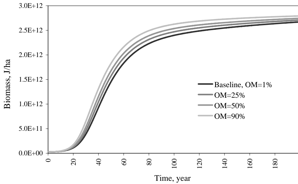
Figure 24. Simulation results of biomass energy storage after increasing initial organic matter storage to 25%, 50% and 90% of its steady state value, showing increased growth rates as the initial organic matter value increases.
