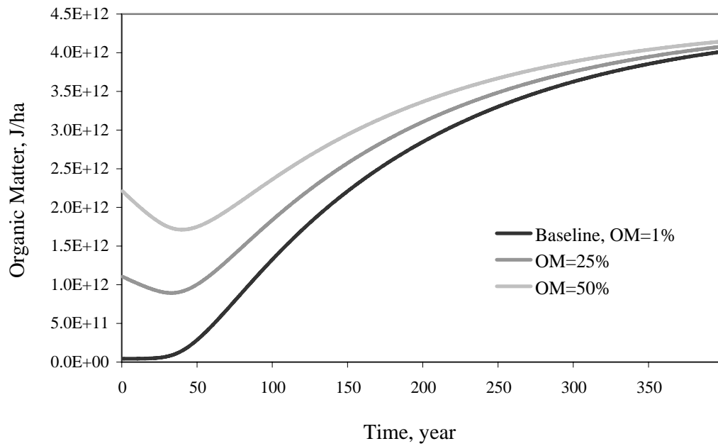
Figure 25. Simulation results of organic matter energy storage after increasing initial organic matter storage to 25% and 50% of its steady state value, showing increased growth rates of organic matter.
