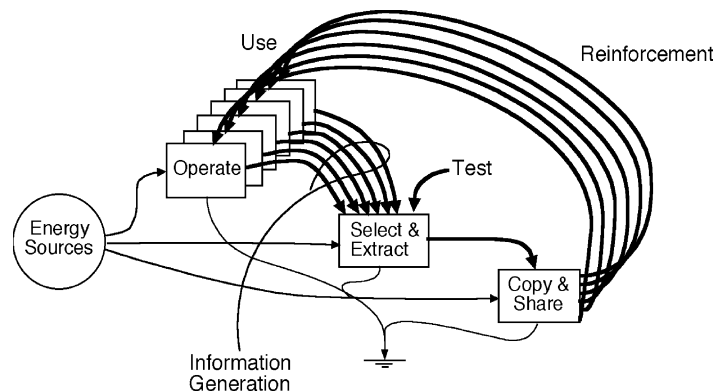
Fig. 1. Diagram illustrating the cycle of generation, selection, sharing, and loop reinforcement through use necessary to maintain and generate new information. (after Odum, 1996).
