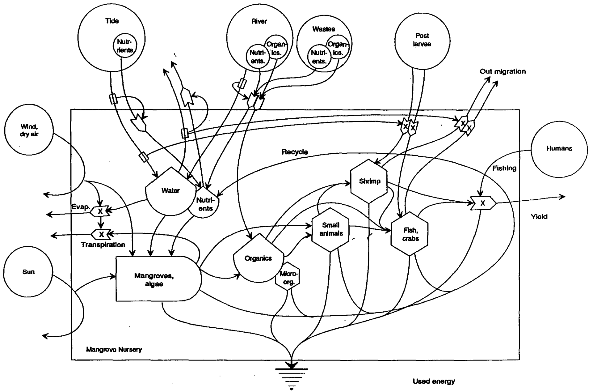
Figure 17. Energy systems diagram of the mangrove nursery ecosystem .
