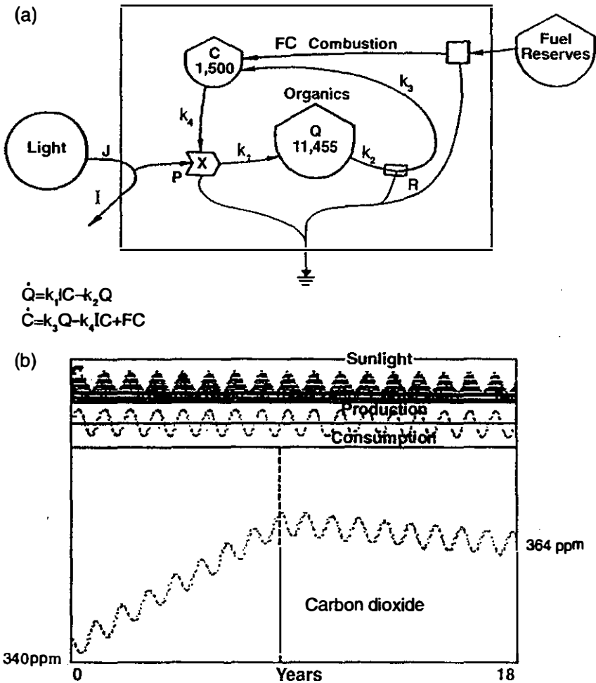
Figure 14.17. Minimodel LANDCO2 of terrestrial processes and atmospheric carbon dioxide without the sea. (a) Energy system diagram. Abbreviations: C , carbon dioxide concentration; Q , organic storage; R , respiration; X , multiplication; J , solar energy inflow; I , remaining energy; k_s , transfer coefficients; P , production; FC , fuel combustion. Equations: I = J/(1 + k_0C) ; dC/dt = R + FC - P ; dQ/dt = P - R , where P = k_1JC , k_1 = k_4 , R = k_2Q , and k_2 = k_3 . (b) Simulation of carbon dioxide resulting from production, consumption, and current fossil fuel use ( FC ). Fuel use was turned off after 8 years.
