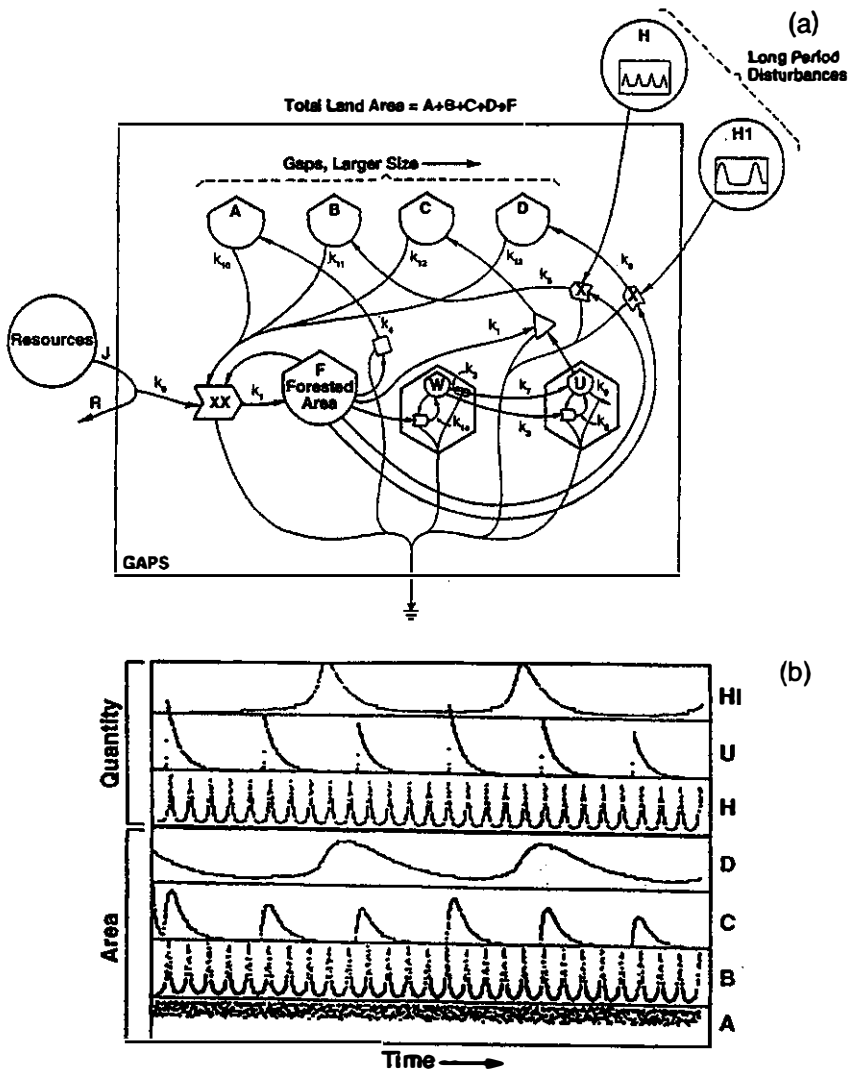
Figure 14.11. Model of gap generation and restoration in a tropical forest, GAPS. (a) System diagram. Abbreviations: A, area of tree-size gaps; B, area of multitree gaps; C, area of several-hectare gaps; D, area of major clearings; U, predator-prey type of oscillatory, epidemic-generating gaps within the forest; F, area in forested cover; TA, total area; G, total gap area; H and H 1 , outside factors with long-period oscillations; Q, wood; Q 1 , competing biomass; J, input of light; R, remaining light unused; k, transfer coefficients; X and XX, multipliers; M, state variable. Equations: G = A + B + C + D ; F = TA - G ; R = J/(1 + k_0G) ; dA/dt = k_4F - k_{10}AR ; dB/dt = k_5FU - k_{11}BR ; dC/dt = k_1U - k_{12}CR ; dD/dt = k_6FH - k_{13}DR ; dU/dt = k_7W + k_8WU^2 - k_9U ; dW/dt = k_{14}FW - k_2W - k_3WU^2 . Equation pairs used as outside oscillating driving functions: dQ/dt = k_{20}M - k_{21}Q - k_{22}QH_1^2 ; dH/dt = k_{21}Q + k_{22}QH_1^2 - k_{23}H ; dQ_1/dt = k_{20}M - k_{21}Q_1 - k_{22}QH_1^2 ; dH_1/dt = k_{21}Q + k_{22}QH_1^2 - k_{23}H_1 . (b) Simulation of GAPS to show growth and pulsing with time; (c) results of simulation with GAPS plotted on a graph of quantity and position in the hierarchy. Continued.
