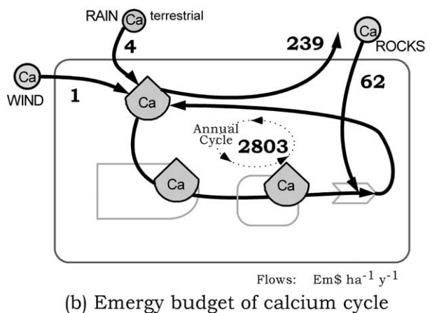
Fig. 3. Systems diagram of calcium cycle at the Coweeta forest (a) and its energy budget (b).
